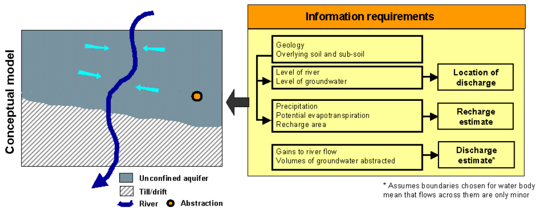
Figure 7: Schematic illustration of a simple conceptual model/understanding of a body of groundwater in which the only significant groundwater discharge is to a river [i.e. the groundwater body has been delineated in such a way that any flows across its boundaries are negligible 21 ].
