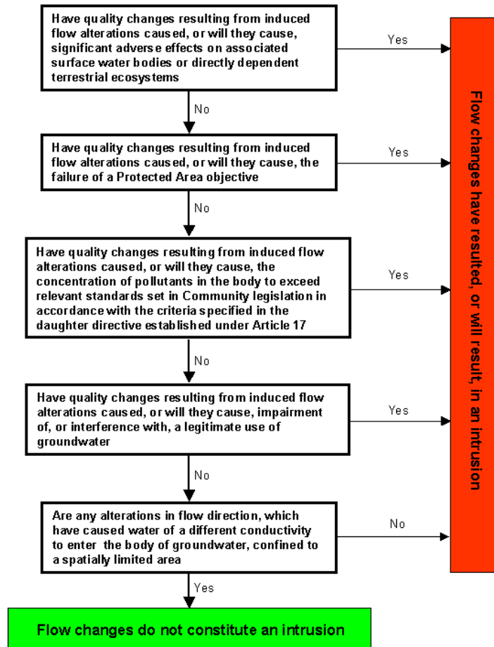
Figure 14: Criteria for defining a saline or other intrusions into groundwater bodies. Where one of the intrusions defined in the figure occurs, a body of groundwater will fail to achieve good quantitative status and good chemical status.
